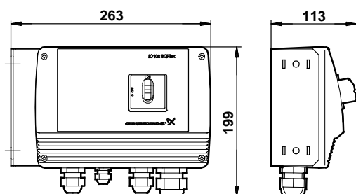
Fig. 27 Dimensions, IO 102
