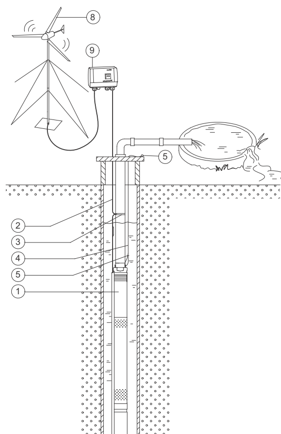
Fig. 11 SQFlex Wind
