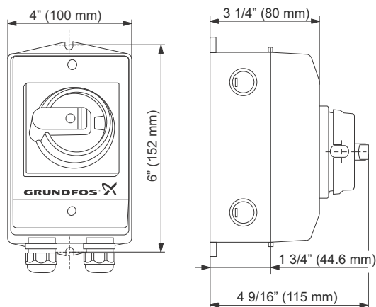
Fig. 23 Dimensions, IO 50
